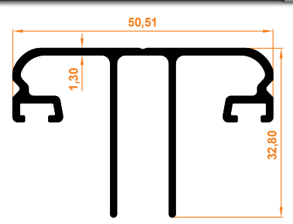
Cam Çita Profili Glass Strip Profile
