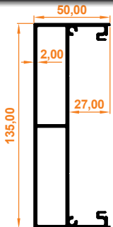
Destek Kutu Profili Reinforcing Box Profile
