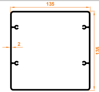
Ayak Profili Leg Profile
