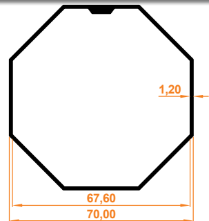
Sac Tambur Borusu Sheet Drum Pipe
