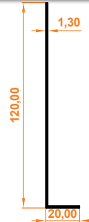
20x120 Köşebent 20x120 Angle Bracket
