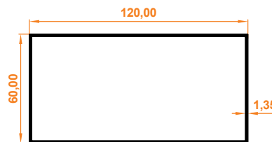
60x120 Kutu Profil 60x120 Box Profile
